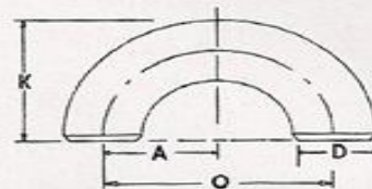
180° SHORT RADIUS RETURN
