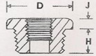
HEXAGON HEAD BUSHING
